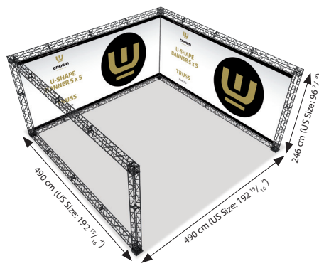
Model 773 / UCT15BM773 Truss U-Shape 5 x 5
