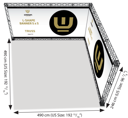
Model 772 / UCT15BM772 Truss L-Shape 5 x 5
