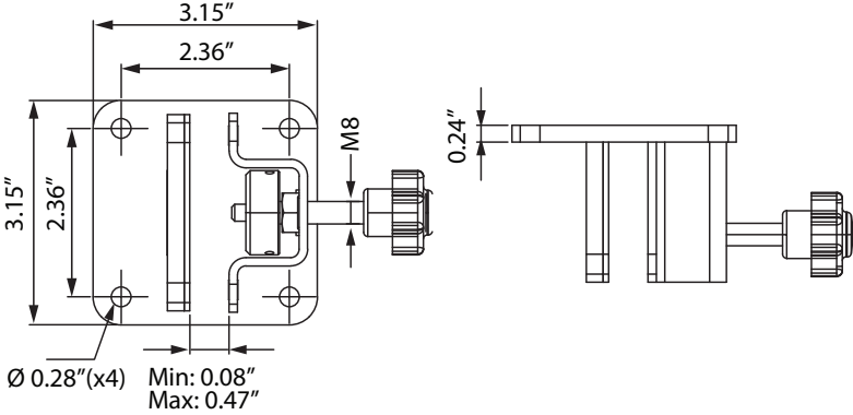
Ceiling Mounting
